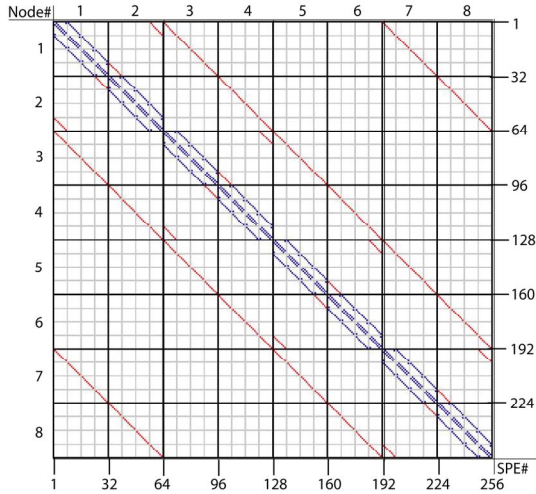
Figure 4. Communication pattern of MD.
