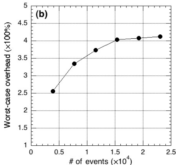
(b) Slowdown due to the profiler
