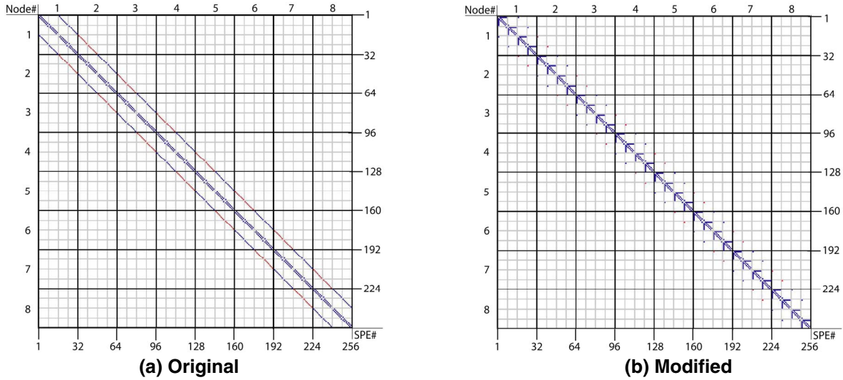
Figure 3. Communication pattern of Sweep3D.
