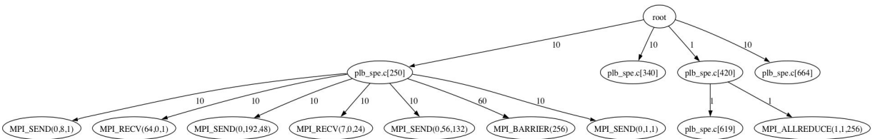
Figure 5. Function call graph for LB.
