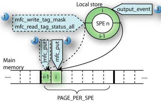
Figure 1. Operation of the profiler double-buffering implementation.
