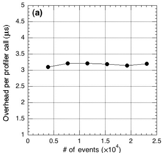
(a) Average cost per profiler call
